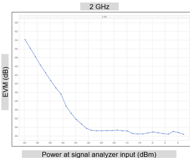
Figure 2. 5GNR FR1, 2.0 GHz carrier, 100 MHz single carrier, 256 QAM, 30 kHz SCS, DC Punc off
